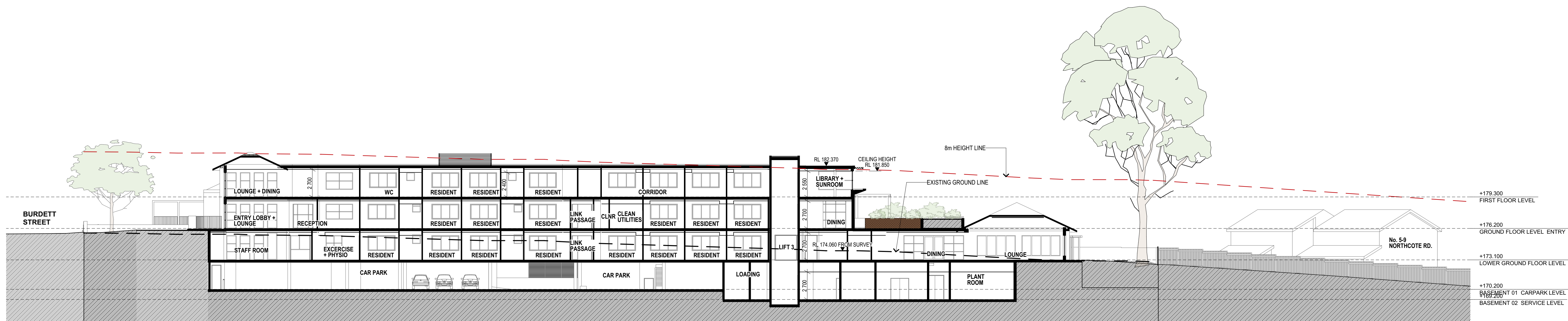
SECTION B
